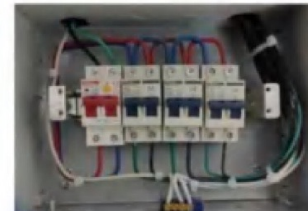
Switchbox
