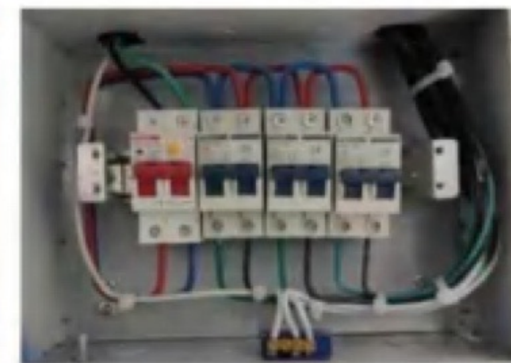
Switchbox
